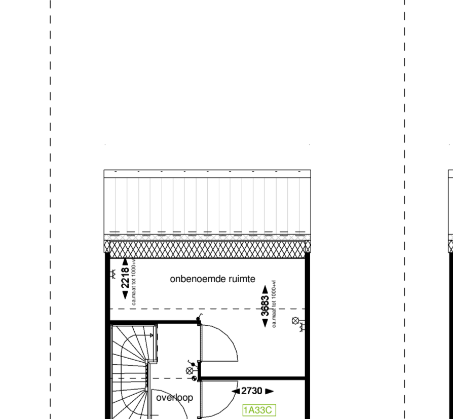
Optie C11.1: Principe zolderindeling bnr: 56, 58, 60, 61, 64, 86, 87
