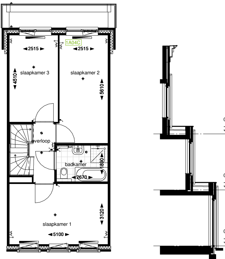
Optie C11.2: Principe zolderindeling bnr: 57, 59, 61, 62, 64, 82, 83, 90, 91, 94, 95, 96, 99
