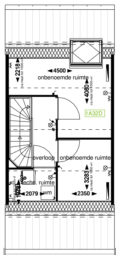
Optie D11.1: Principe zolderindeling bnr: 137, 139
