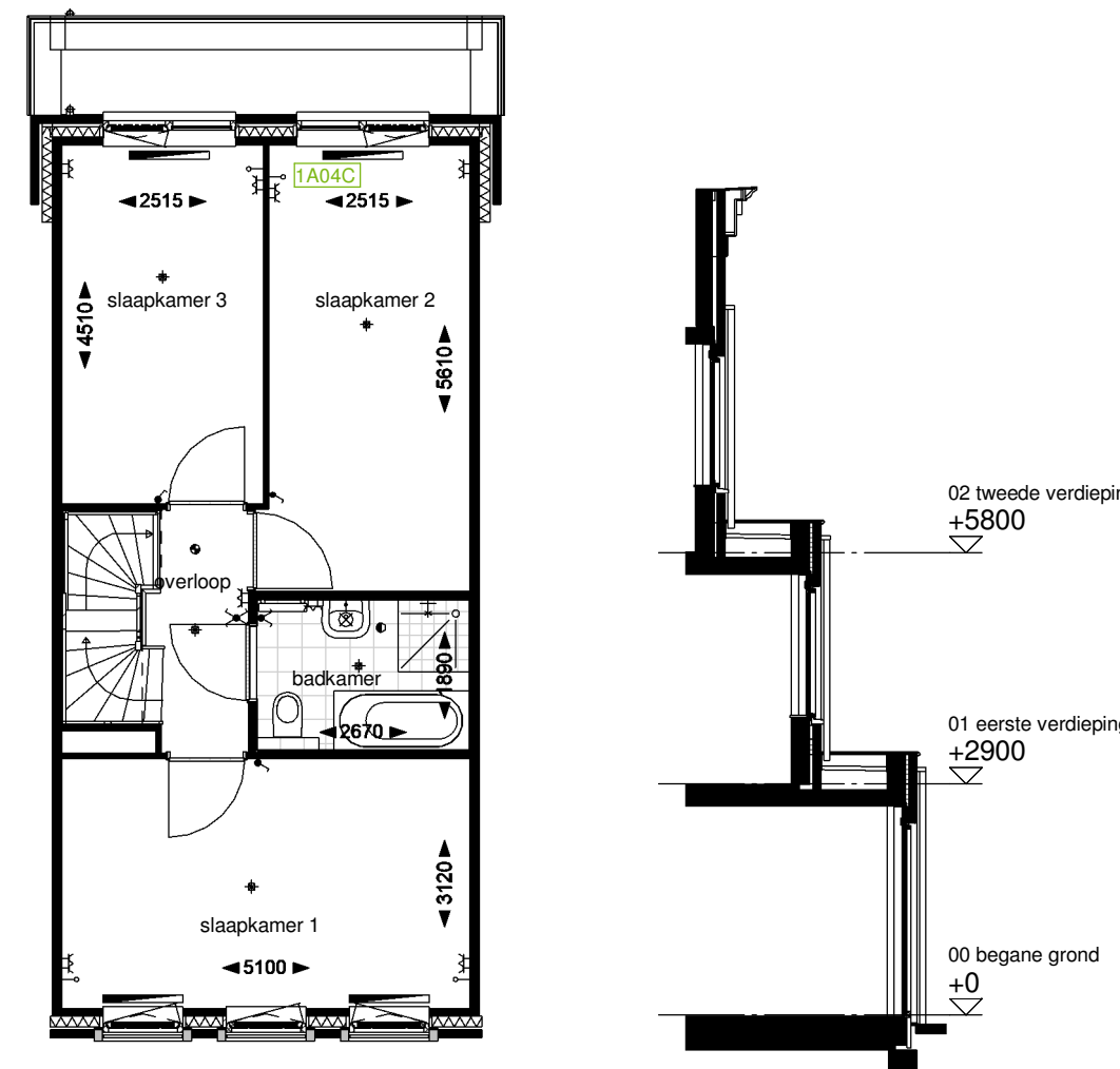
Optie C11.2: Principe zolderindeling bnr: 116, 118, 120, 122, 124 t/m 126, 128, 130, 132, 133, 134
